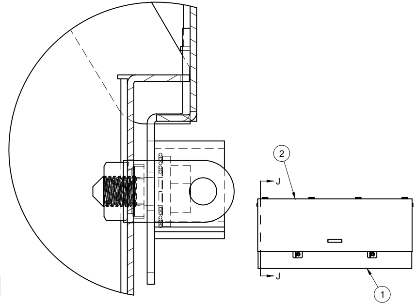
DETAIL N SCALE 1:1.5
